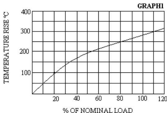
TEMPERATURE RISE AT CONSTANT LOAD
